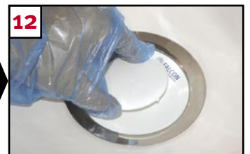
12 Snap the diverter shield into place
